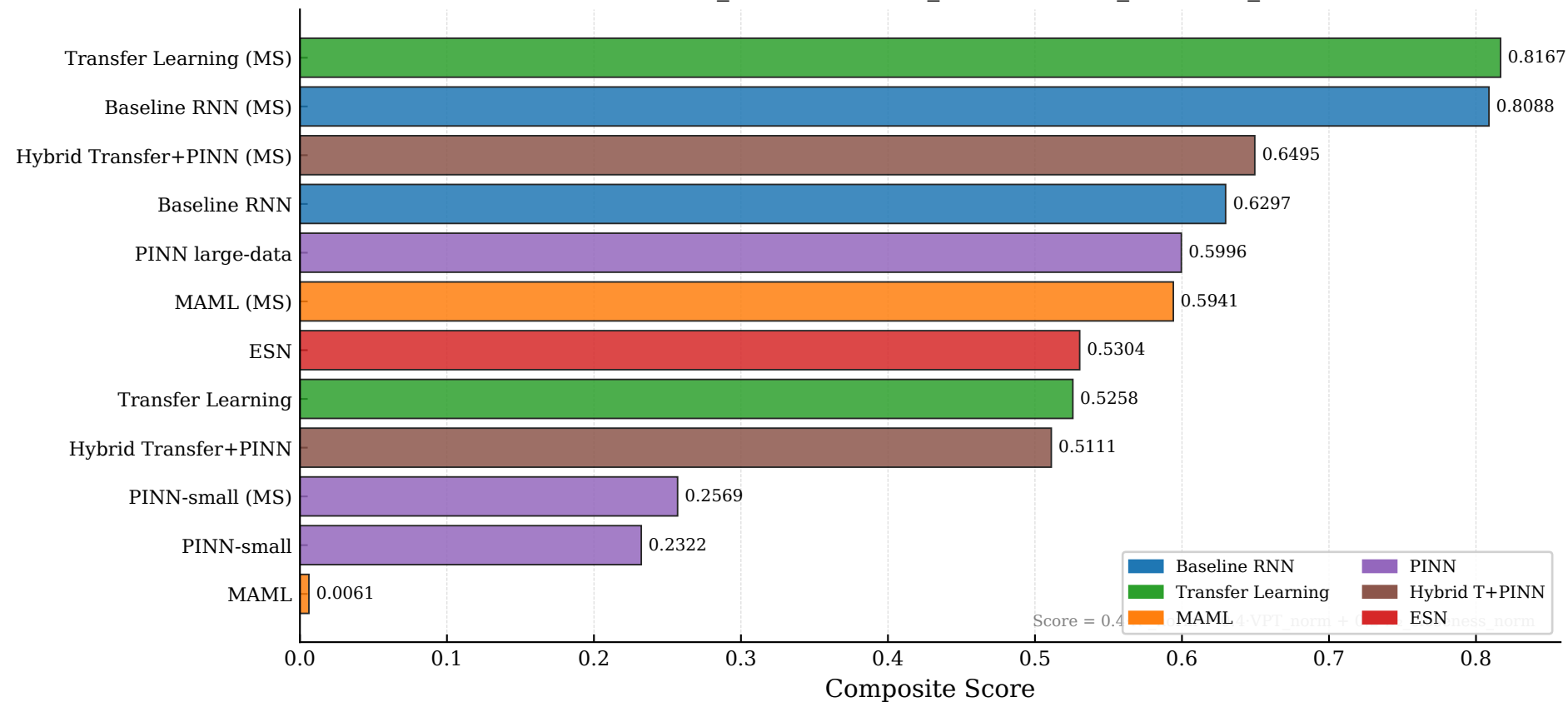
KS — Three-Metric Composite Leaderboard \text{Score} = 0.4 \cdot R^2_{\text{norm}} + 0.4 \cdot \text{VPT}_{\text{norm}} + 0.2 \cdot D_2_{\text{closeness}_{\text{norm}}}
